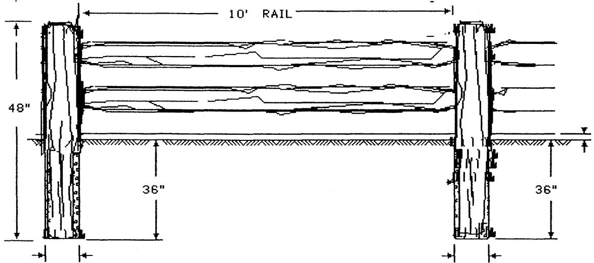
(ELEVATION VIEW)
